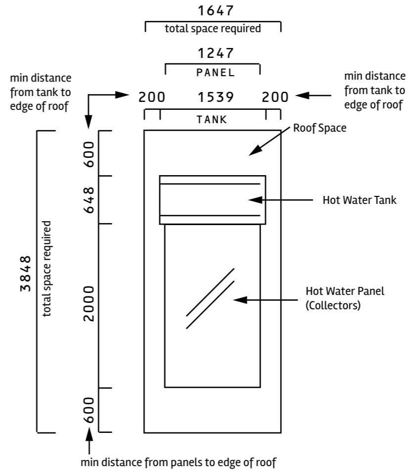
B Roof mounted solar hot water (single panel)
